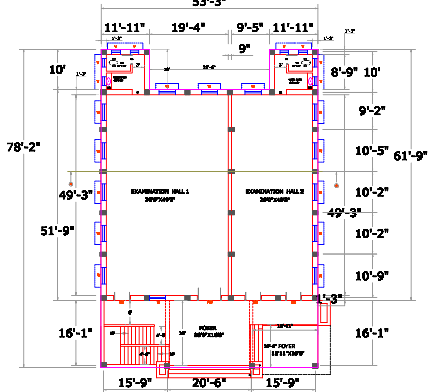
GROUND FLOOR PLAN (WEST FACING)
